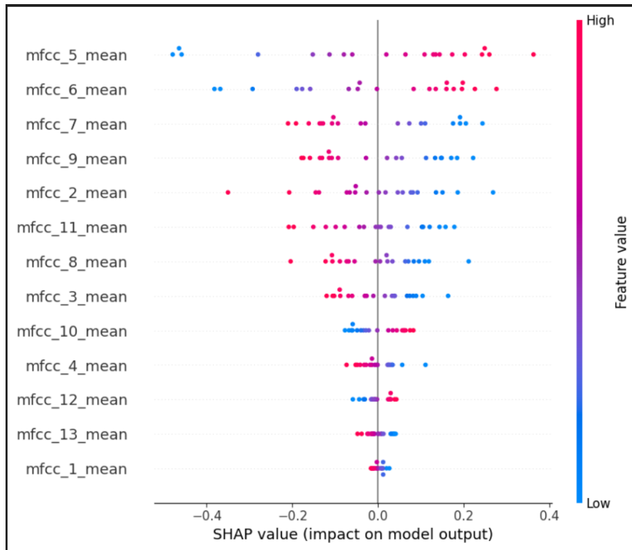
Figura 30: Shap global MFCCs.
