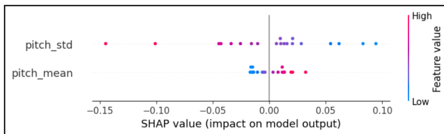
Figura 26: Shap global pitch.
